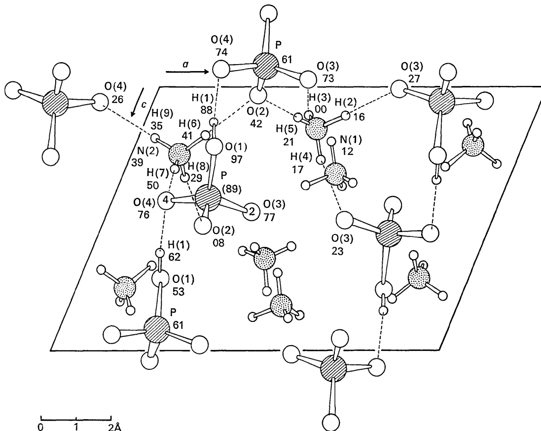
Fig. 1. (\text{NH}_4)_2\text{HPO}_4 , viewed along [010] . The heights of selected atoms are indicated in fractional coordinates ( \times 100 ).
